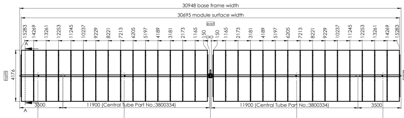
DEGER S100-PF-DR With Driven Pile Foundation (1)
